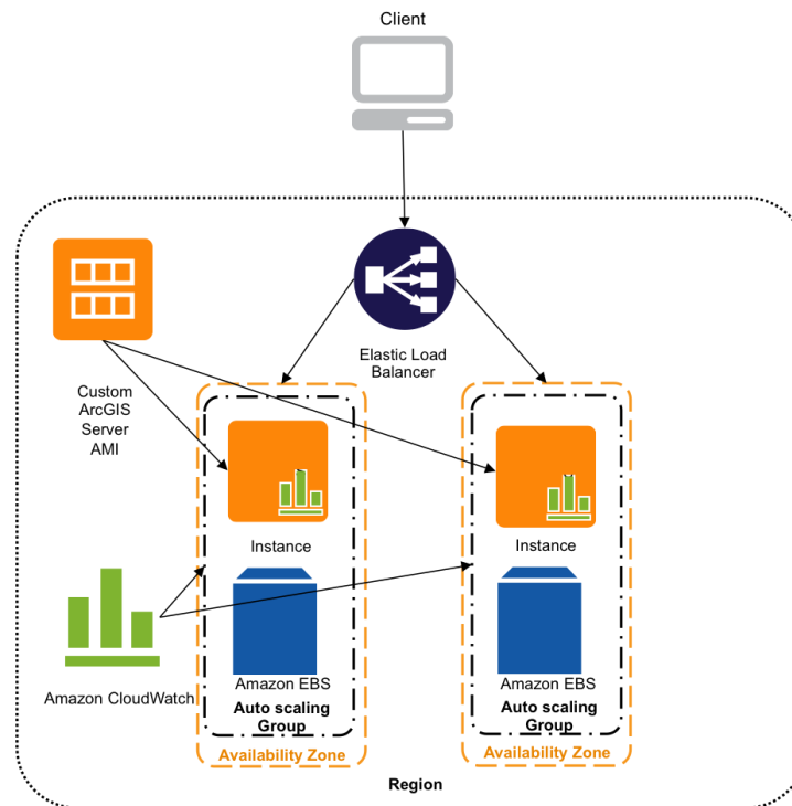
Figure 4: Custom ArcGIS for Server in AWS
